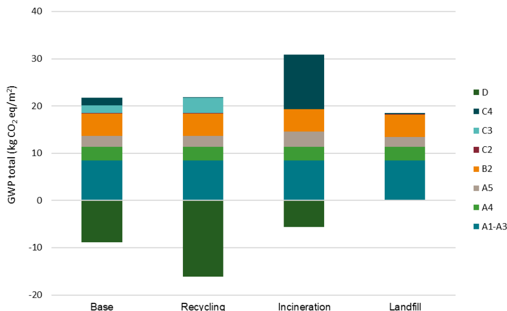
Figure 3: Contributions to GWP for each waste management scenario for SPC Click DL (excludes B4)
