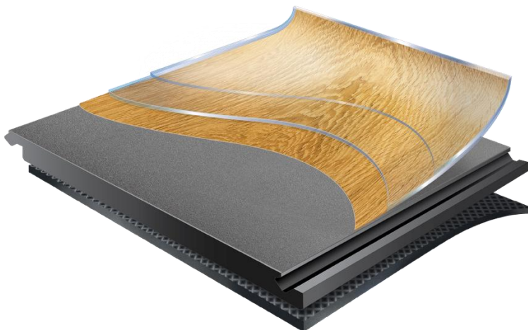
Figure 1: Construction of Novalis Stone Polymer Core (SPC)
