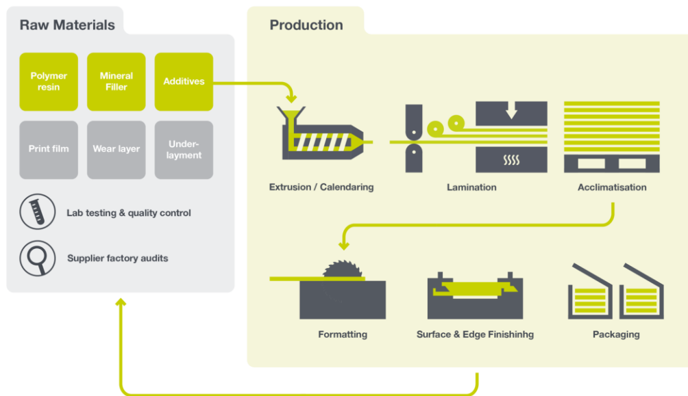
Figure 2: Production Process of Novalis Stone Polymer Core (SPC)
